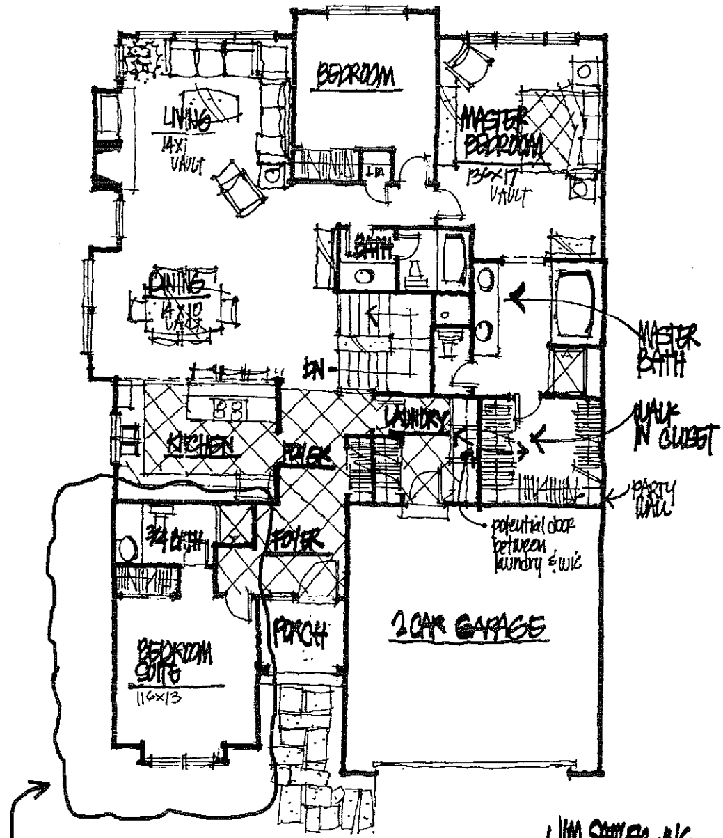
OPTIONAL FRONT BEDROOM PLAN 4 3/4 bath.
